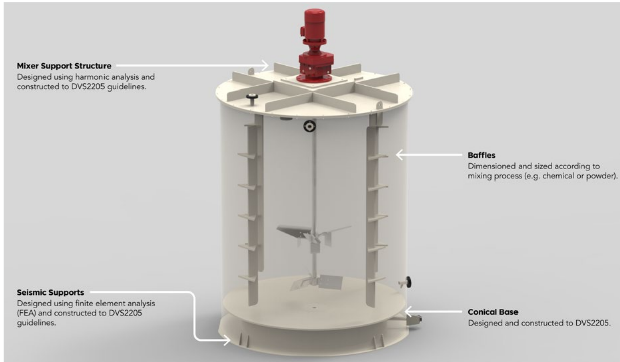
A Custom fabricated HDPE tank with roof mounted agitator designed to clients specifications and complete with internal conical base.
